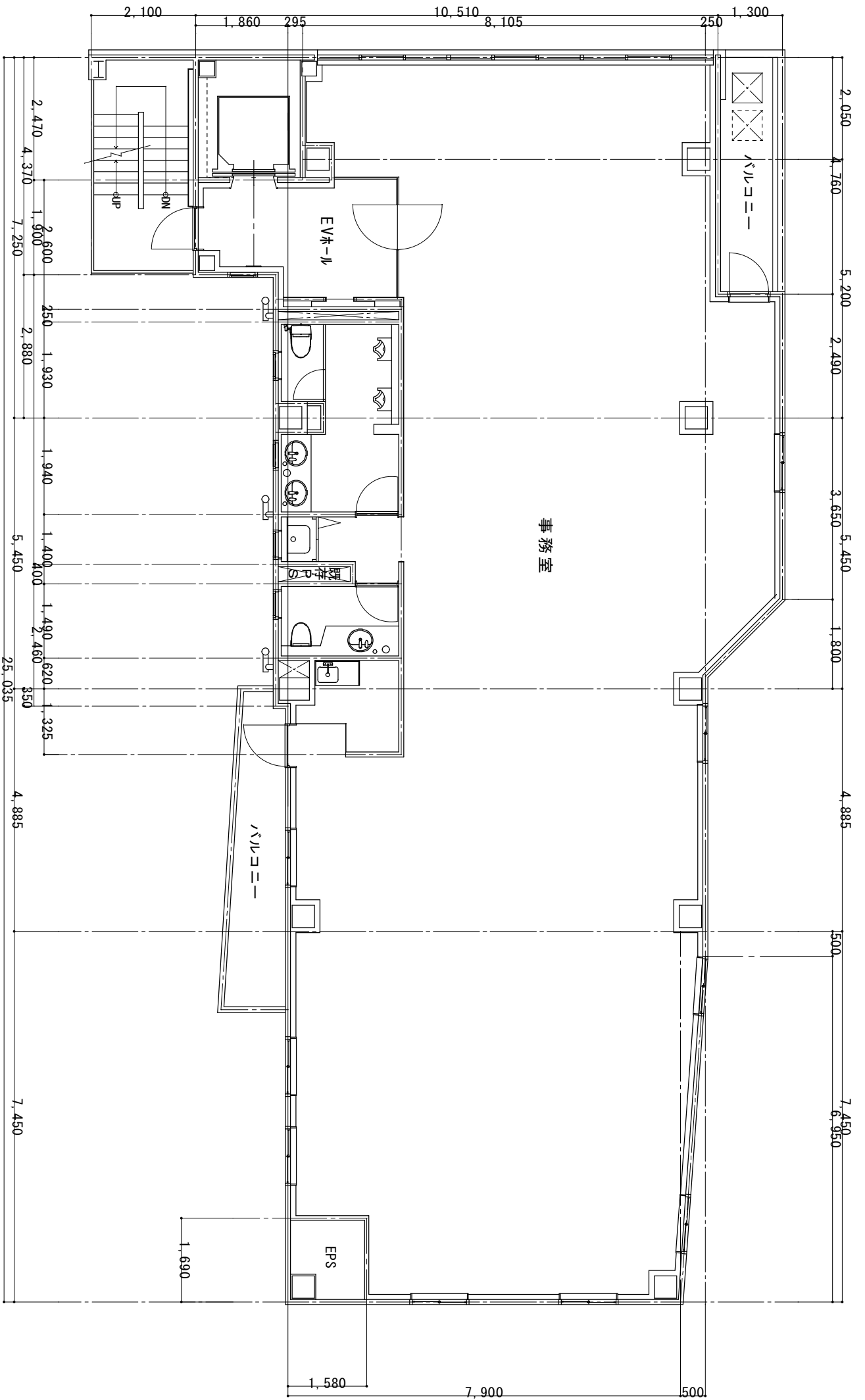
9階平面図 S = 1/100
